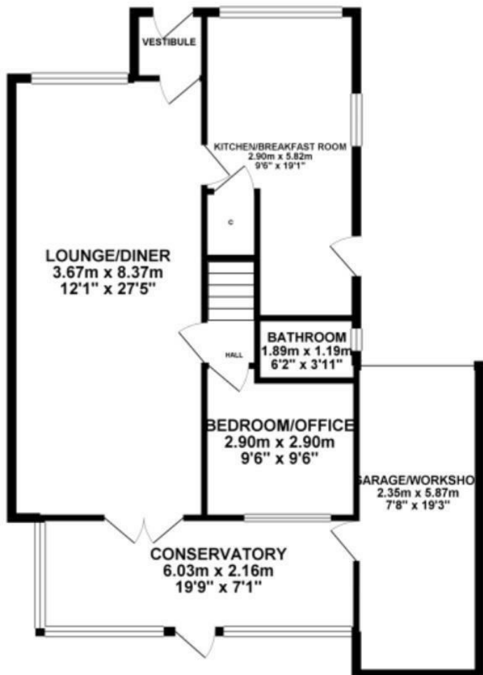
GROUND FLOOR 87.15 sq. m. ( 938.07 sq. ft. )
